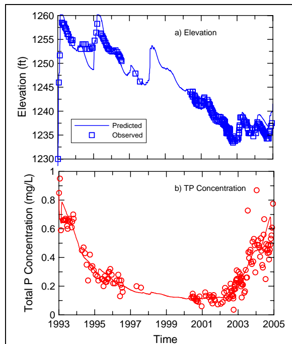
Fig. 11. Predicted and observed: a) lake surface elevation and b) TP concentration.
